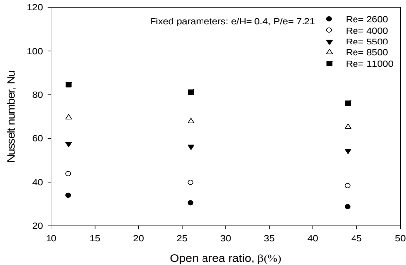
Figure 13 Variation of Nusselt number with open area ratio ( \beta ) at different Reynolds number.
