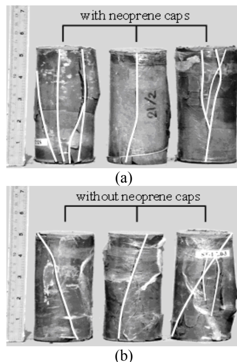
Figure 3. Failures of rock specimens with L/D = 2.0 after testing with (a) and without (b) neoprene caps. Induced fractures are highlighted with white lines.
