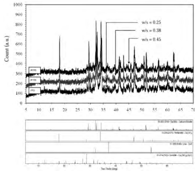
Figure 7 X-ray diffraction of the pastes of 0.25, 0.38 and 0.45 after applying MW power of 100 watt for 30 minutes.
