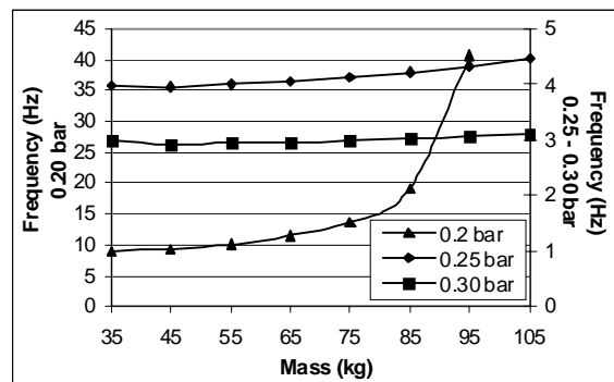
Figure 5 The natural frequency of the vibration isolation mechanism for applied air pressure of 0.20 bar (left axis), 0.25 and 0.30 bar (right axis).
