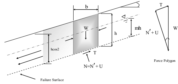
Figure 3 Infinite slop stability analysis model
