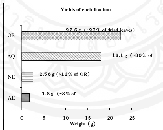
Figure 3 Percentage of yields of each fraction separated by acid-base solvent partitioning from B. lupulina dried leaves.
