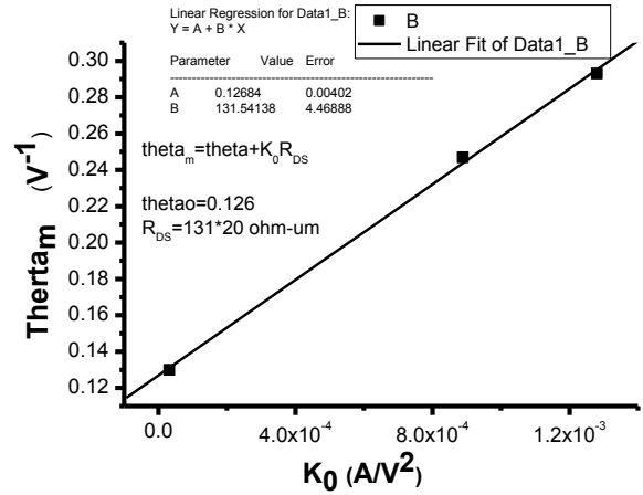
Figure 8. Extracted THETA versus K_o of PMOS devices at 27 °C with drawn gate length of 20, 0.8 and 0.6 \mu\text{m}
