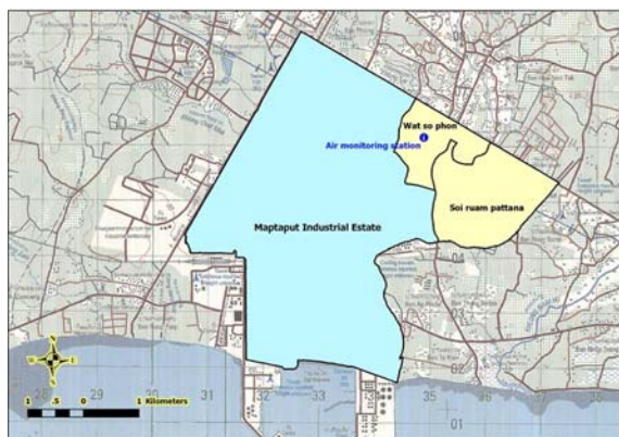
Fig. 1 The studied area showing Soi Ruam Pattana and Wat So Phon communities, the ambient air monitoring station at Map Ta Phut health center, and Map Ta Phut Industrial Estate.
