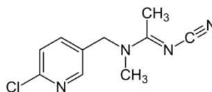
Figure 1 : Acetamiprid chemical structure
