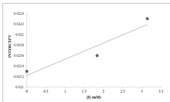
Fig 5. Secondary plot of intercept vs [I] for deduction of K'_1 of 3 against sucrase.
