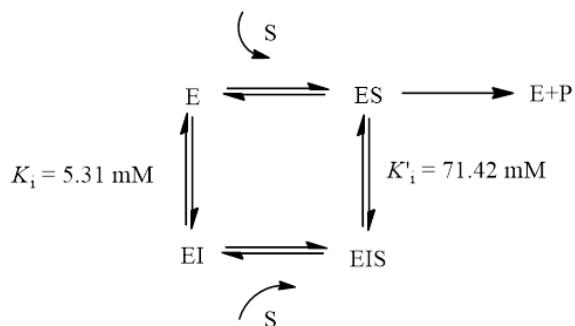
Fig 3. Proposed inhibitory mechanism of 3 against sucrase.
