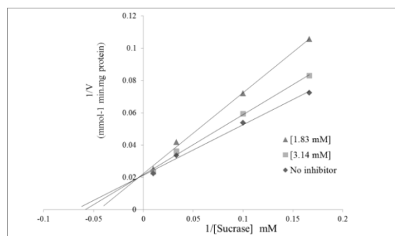
Fig 2. Lineweaver-Burk plots for inhibitory activity of 3 against sucrase.
