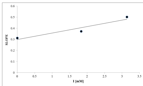
Fig 4. Secondary plot of slope vs [I] for deduction of K_i of 3 against sucrase
