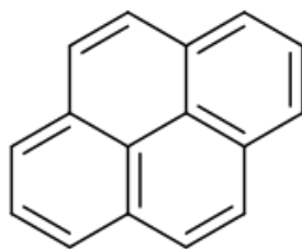
Fig. 1 Formula of 1-hydroxypyrene (C 16 H 10 ) Napthalene (C 10 H 8 ) (Marcia, 2001)
