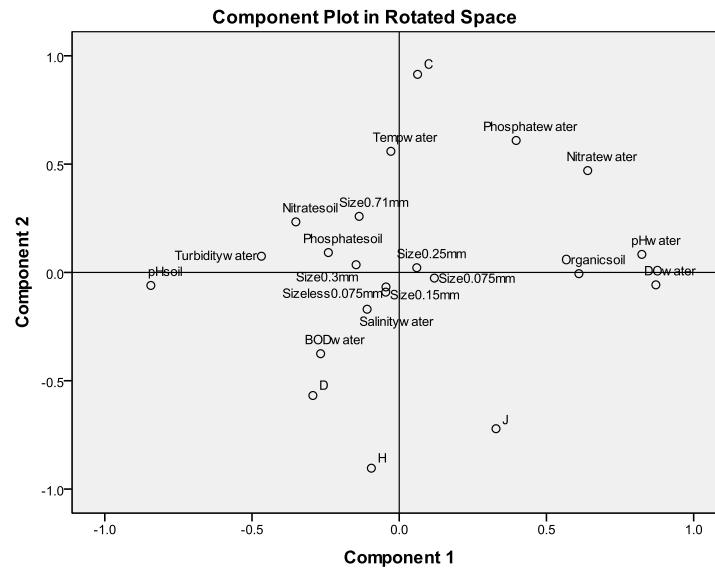
Fig. 3 PCA of relationship between biodiversity indices and ecological characteristics
