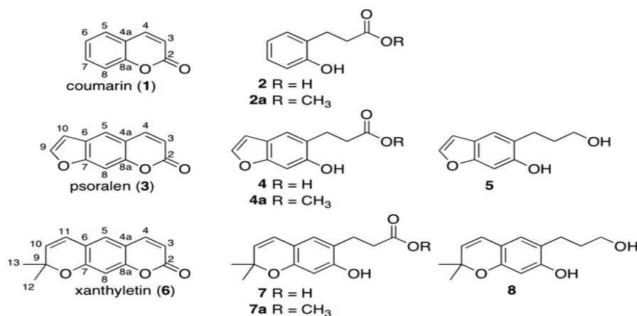
Fig. 1. Chemical structures of coumarin, psoralen, and xanthyletin derivatives
