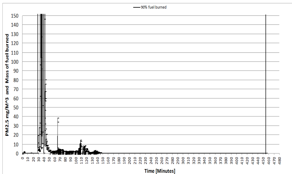
Fig. 10. PM 2.5 emissions profile for a BLUD Imbaulta.
