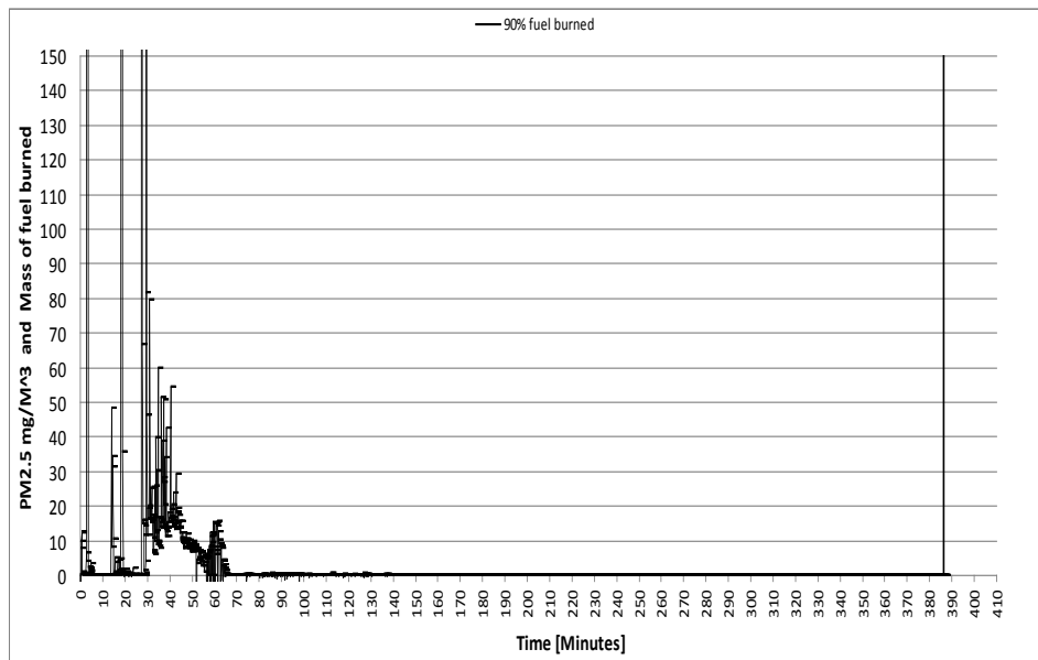
Fig. 13. PM_{2.5} emissions profile for a TLUD Imbault.
