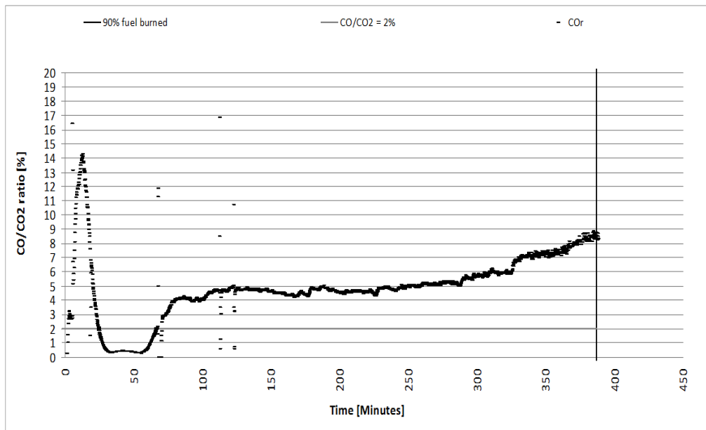
Fig. 11. CO/CO 2 emissions profile from the TLUD method.
