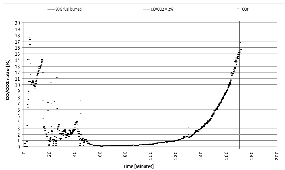
Fig. 14. CO/CO_2 profile for the SeTAR BLDD cookstove over an entire sequence.
