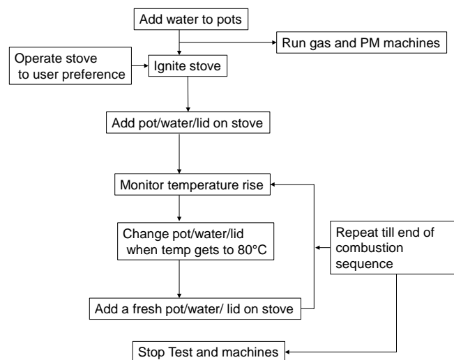
Fig. 5. A schematic of the testing sequence of the HTP.
