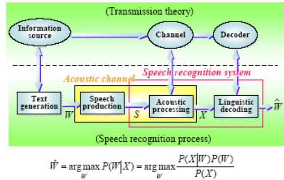
Fig.2: Statistical modeling framework of speech production and recognition system based on information transmission theory.
