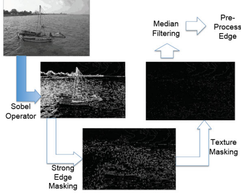
Fig.2: Illustration of Pre-Process Stage. The first input is a grayscale image transformed from original Sailing1 category image from LIVE JPEG Database. A Sobel Operator applied to the input and generate the edge image. The edge image then is masked (spatial masking process). After the spatial masking process, the image undergo a texture filtering process. Additionally, a median filter is applied to the image and the final pre-processed image is generated.
