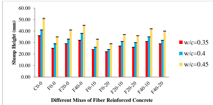
Figure 2. Slump height of different mixes
