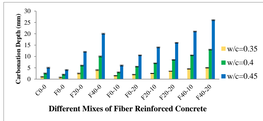
Figure 7. Carbonation depth of hardened concrete at 28 days curing
