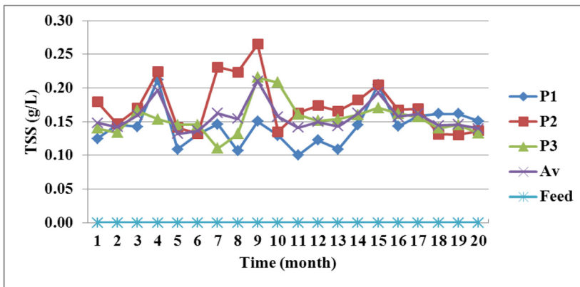
Figure 3. Total suspended solids of feed and reactors.
