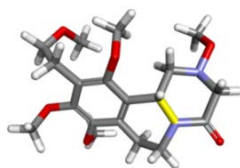
Figure 6. Molecular structure of PZQ derivative substituted with -\text{CH}_2\text{CH}_2\text{OCH}_3 in \text{R}_3 position (G05_R3)
