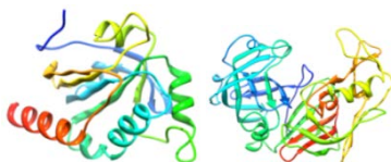
Figure 4. The structures of thioredoxin peroxidase (Left) and aspartic protease (Right)
