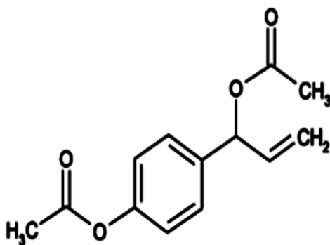
Figure 1 Molecular structure of 1'-Acetoxychavicol acetate (ACA) [3]
