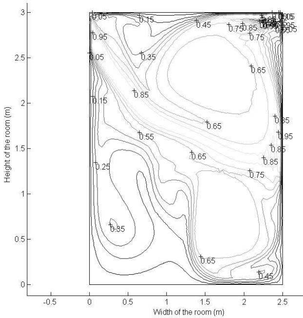
Fig. 2. Contour isotherms.
