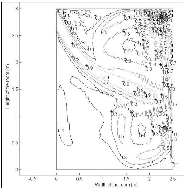
Fig. 3. Contour flow.
