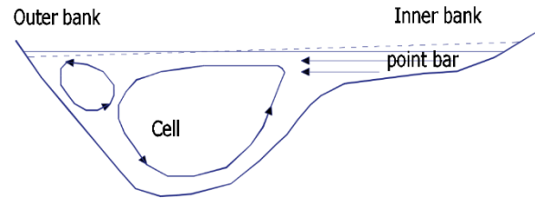
Figure 1 Balance between centrifugal force and pressure gradient.
