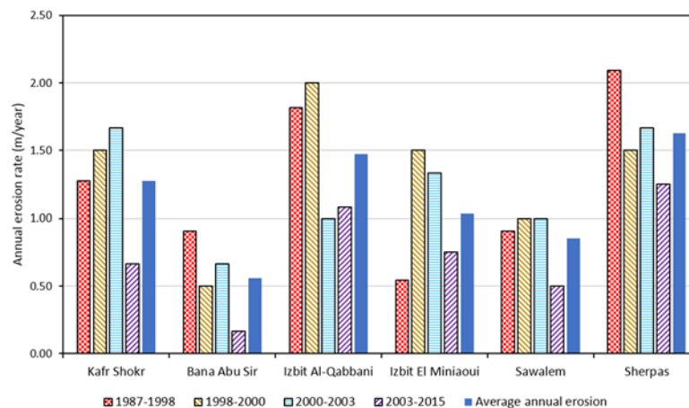
Figure 12 The Annual erosion rate (m/year).
