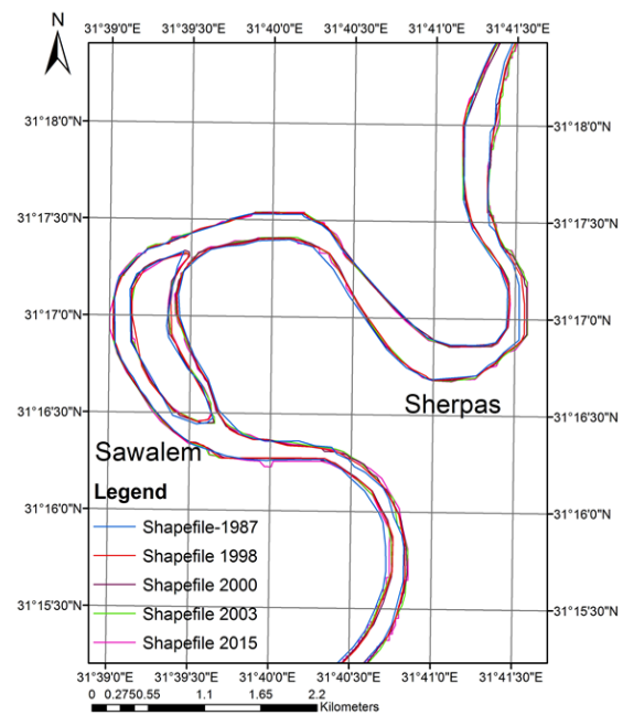
Figure 10 Temporal changes for Sawalem and Sherpas forced bends.
