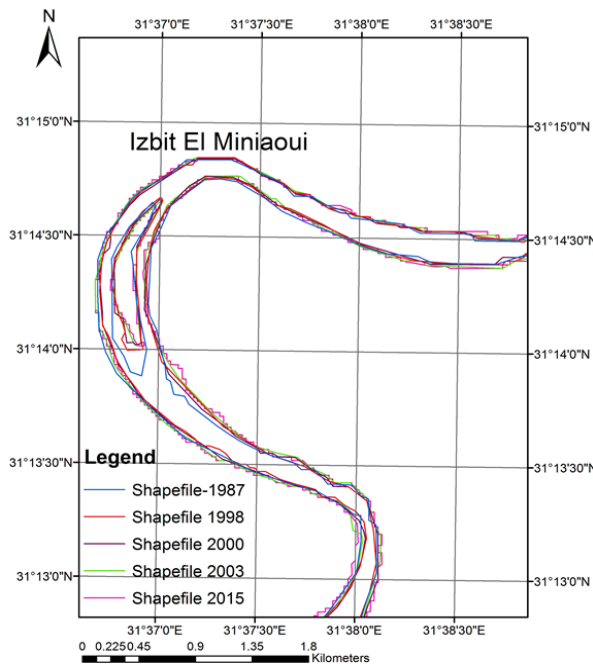
Figure 9 Temporal changes for Izbit El Miniaoui forced.
