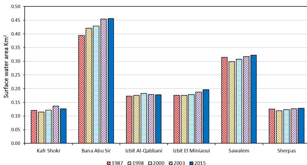
Figure 11 The surface water area of the studied forced bends in km 2 .
