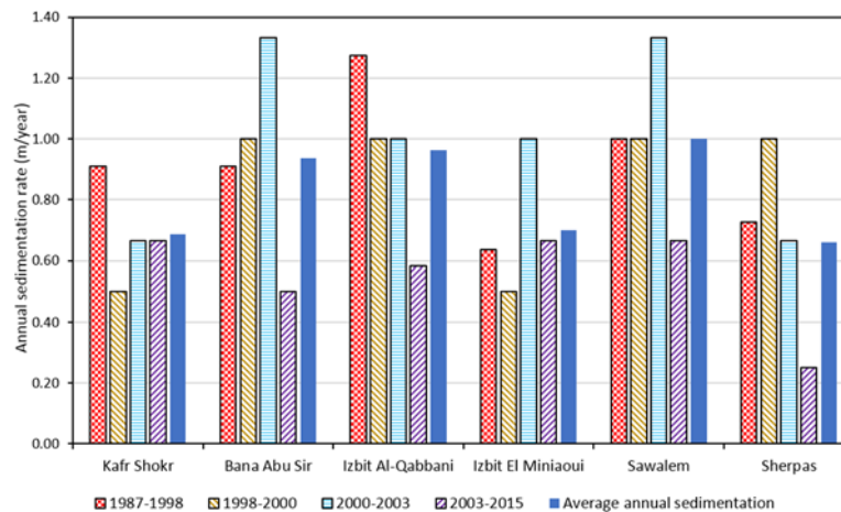
Figure 13 The Annual sedimentation rate (m/year).
