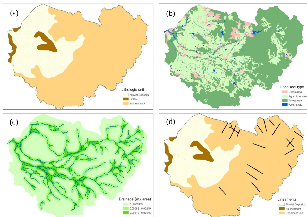
Figure 2 Factors affecting the groundwater recharge: (a) lithology, (b) land use, (c) drainage density ( \text{m}/\text{km}^2 ) and (d) lineament
