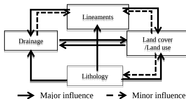
Figure 3 The interactive influence of factors considering groundwater recharge potential [10]
